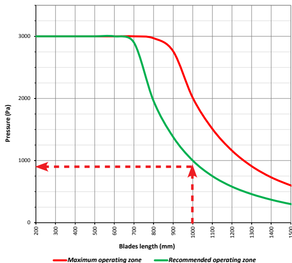
Backdraught damper AR
