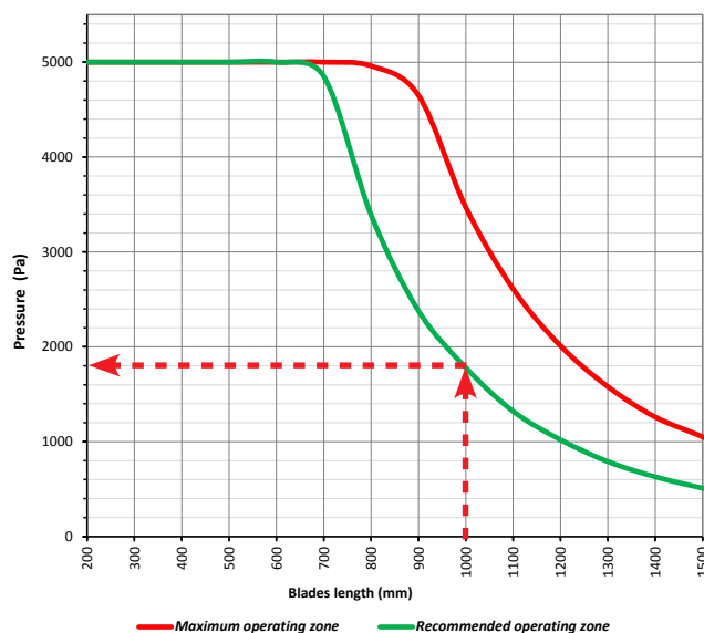
Backdraught damper AE
